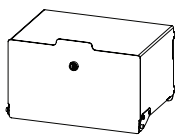
Lock Box Specifications: 14"W x 10"D x 7.5"H Part Number: 73528770
