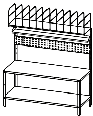
Pack Station Specifications: 72"W x 30"W x 84.5H Weight: 220lbs. Part Number: 76452000
